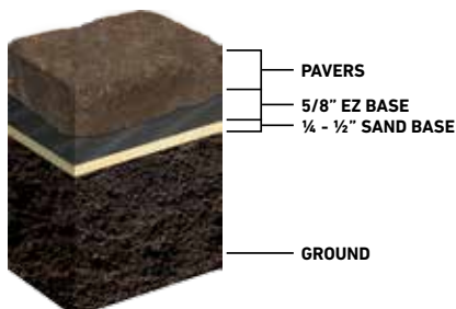
EZ Base® METHOD (Approx. 3\"/>
